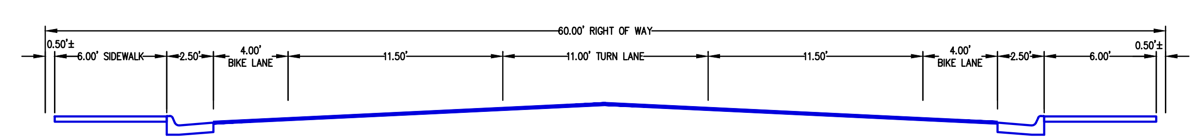
TYPICAL ROADWAY SECTION 1" = 5'
