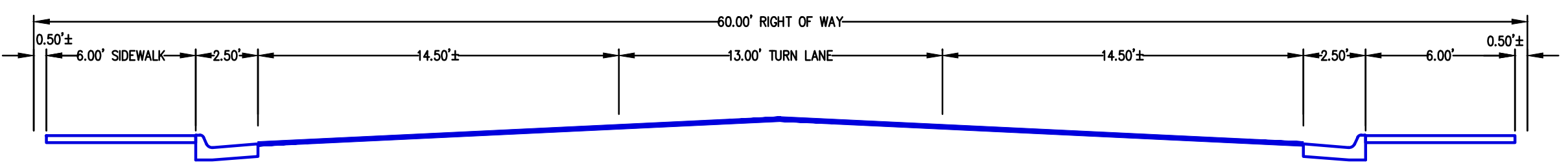
TYPICAL ROADWAY SECTION 1" = 5'
